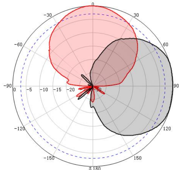
V-Pol- 6.6GHz
