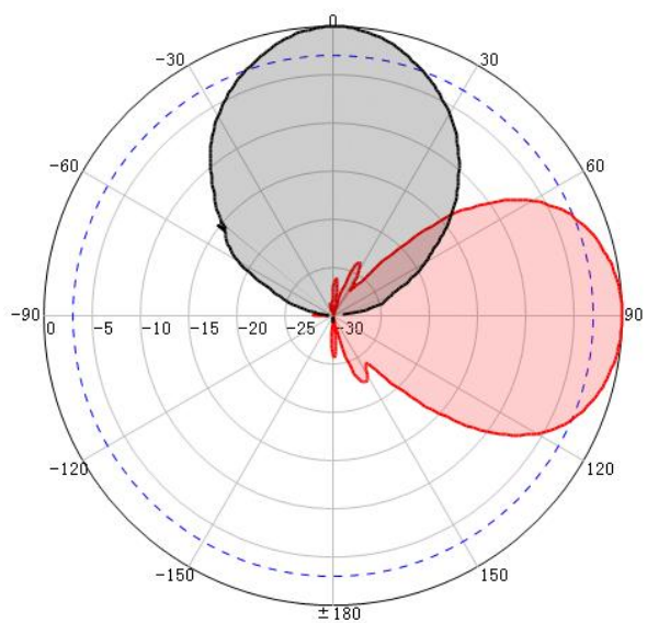
V-Pol- 6.6GHz
