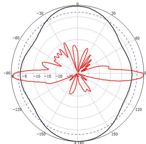
V-Pol @ 2450MHz
