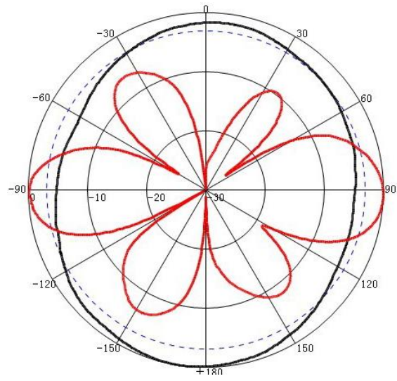
V-Pol @ 2450MHz
