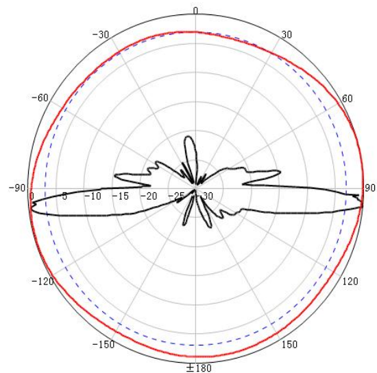
V-Pol @ 5550MHz
