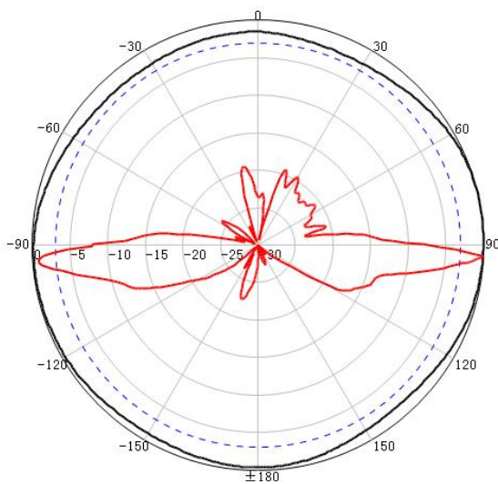
H-Pol @ 5550MHz
