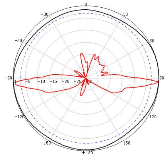
V-Pol @ 5550MHz
