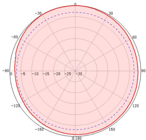
Axial Ratio
