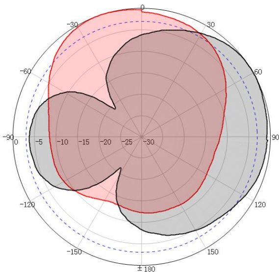
868 MHz
