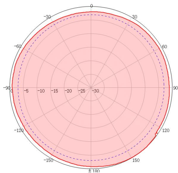
Axial Ratio
