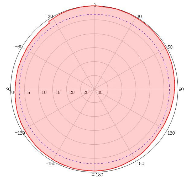
Axial Ratio
