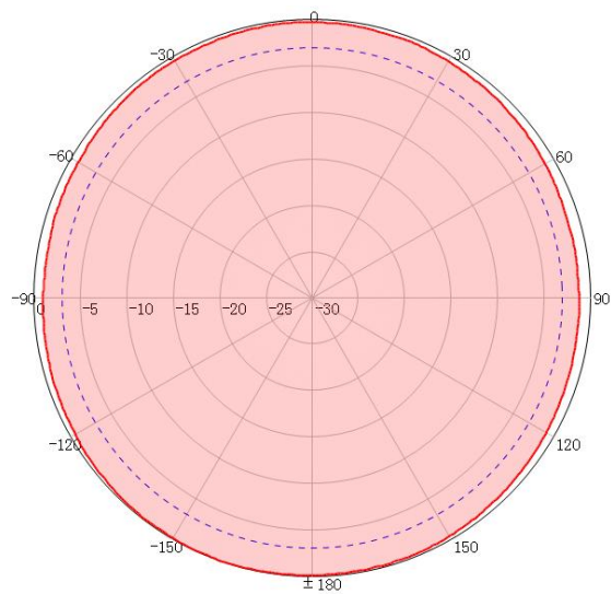
Axial Ratio
