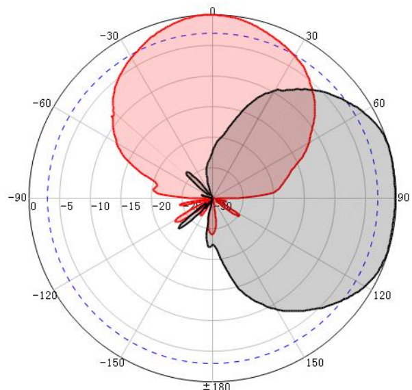
V-Pol- 6.6GHz
