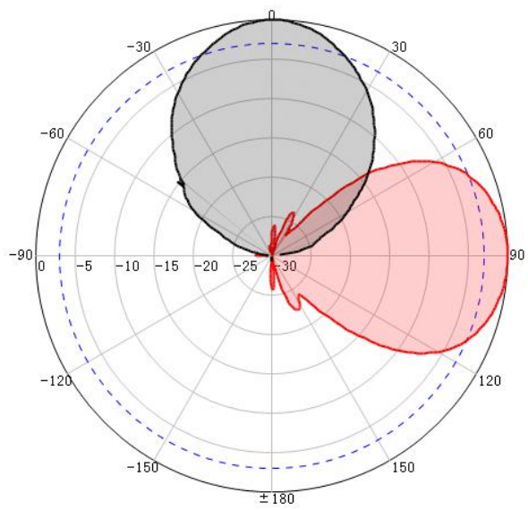
V-Pol- 6.6GHz
