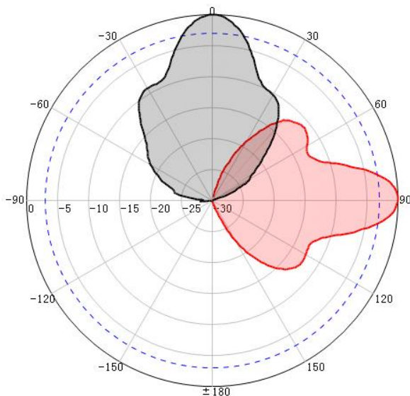
H-Pol – 6.6GHz
