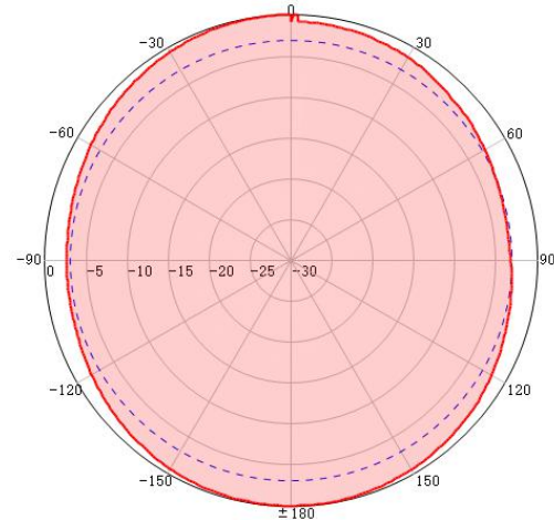
Axial Ratio
