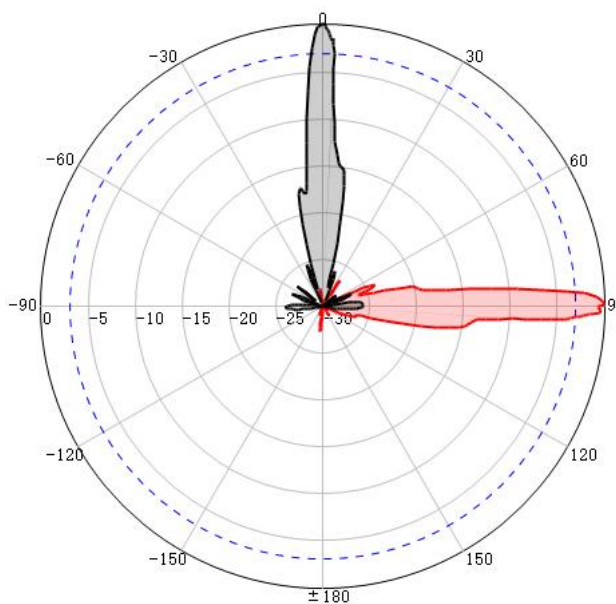
H-Pol @ 4.7GHz
