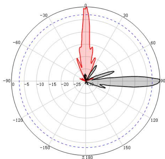
H-Pol @ 4.4GHz
