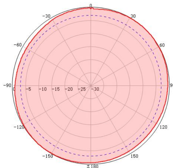
Axial Ratio
